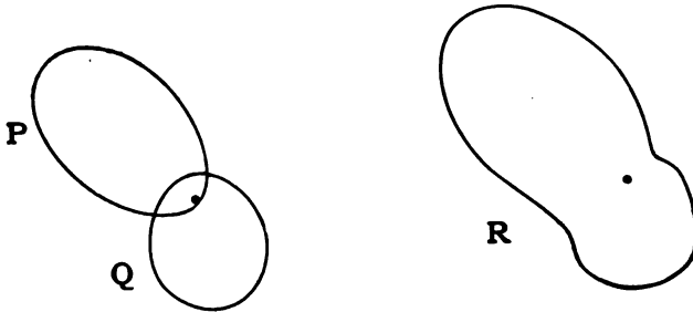
FIG. 7.—Calculated Distributions of Proper Motions.
